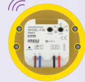
Universal dimmer - MULTI function
